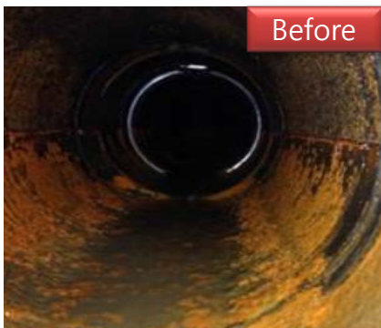
Before chemical cleaning Condensate Line
