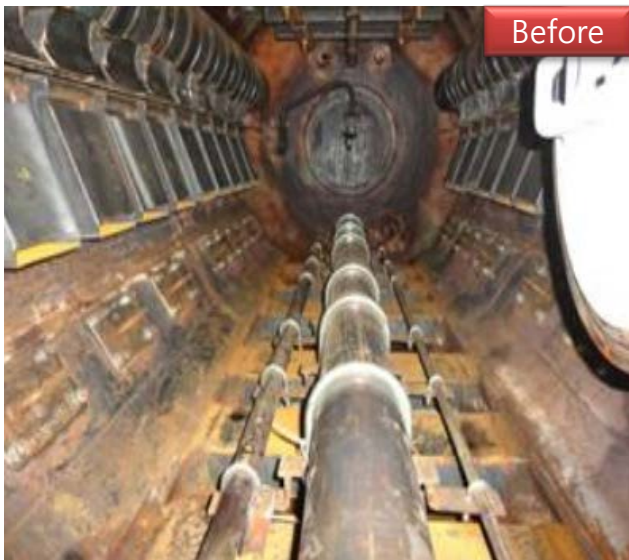
Before chemical cleaning Steam Drum
