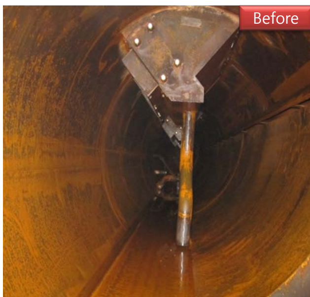
Before chemical cleaning Steam Drum
